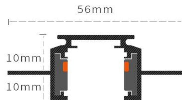
Embedded concealed track N1510/15/20/30-W/B
