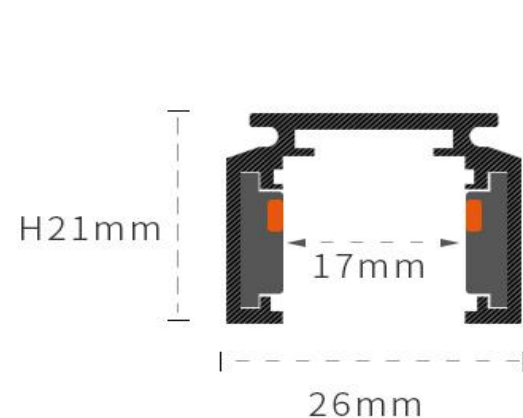
Surface mounted track M1510/15/20/30-W/B
